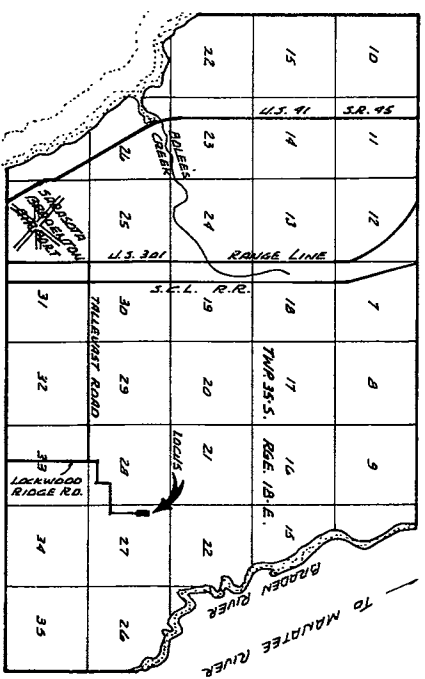
LOCATION MAP
